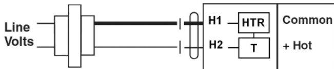
24 VAC Transformer
