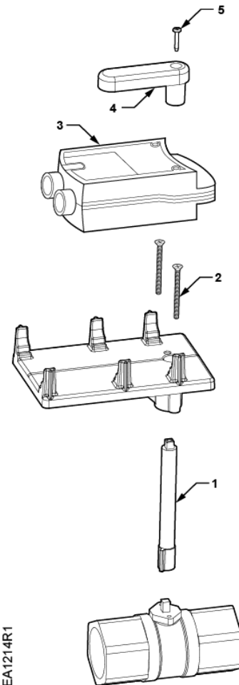
EA1214R1 Figure 5. Order of Assembly.
