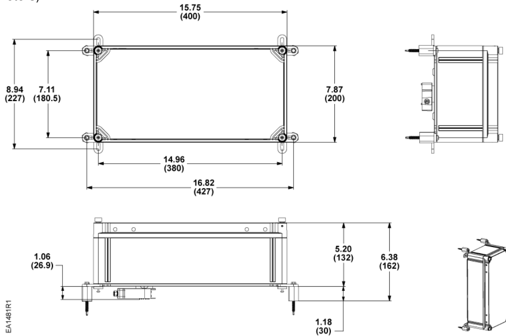
EA1481R1 Figure 13. Dimensions of the ASK75.7U Weather Shield in Inches (Millimeters).
