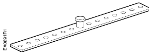
Figure 5. 985-055P24 Anti-rotation Bracket (Mounting).
