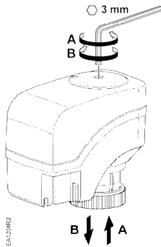
Figure 9. SSA61U and SSA81U Normally Closed.
