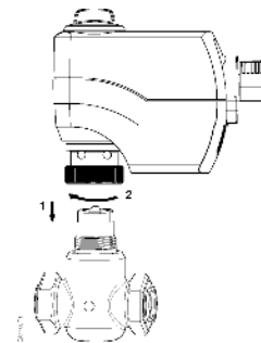
Figure 3. Coupling Actuator to Valve.
