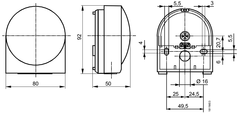
Drilling plan
